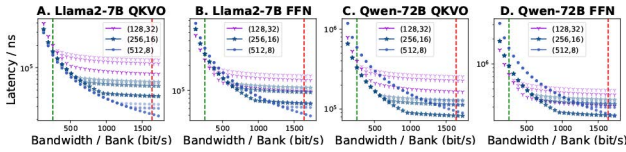
Fig. 22. DSE of SRAM-PIM in CompAir. The lighter dots mark the latency at lower voltages (0.6V-0.8V).
